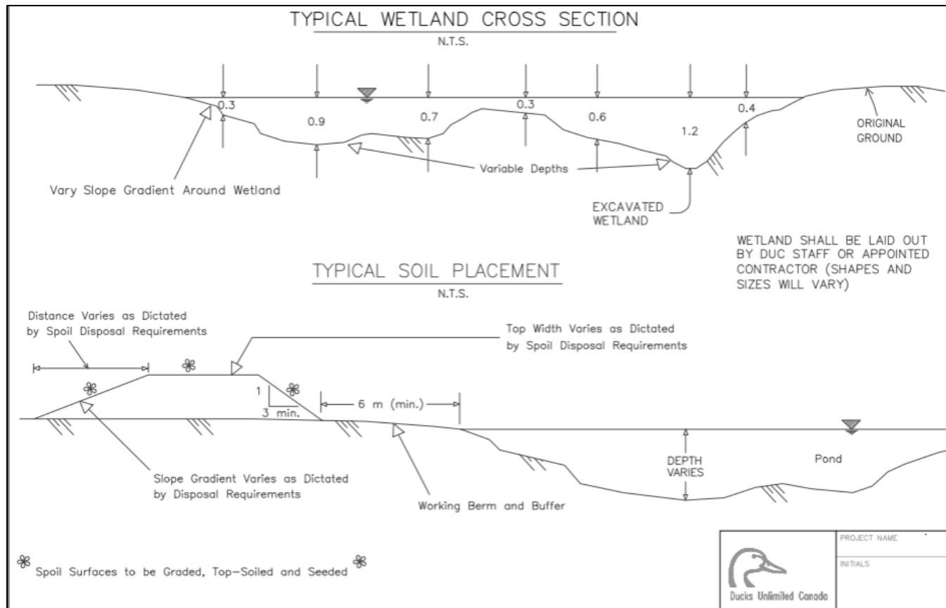
Figure 1: Cross section of a typical excavated wetland
