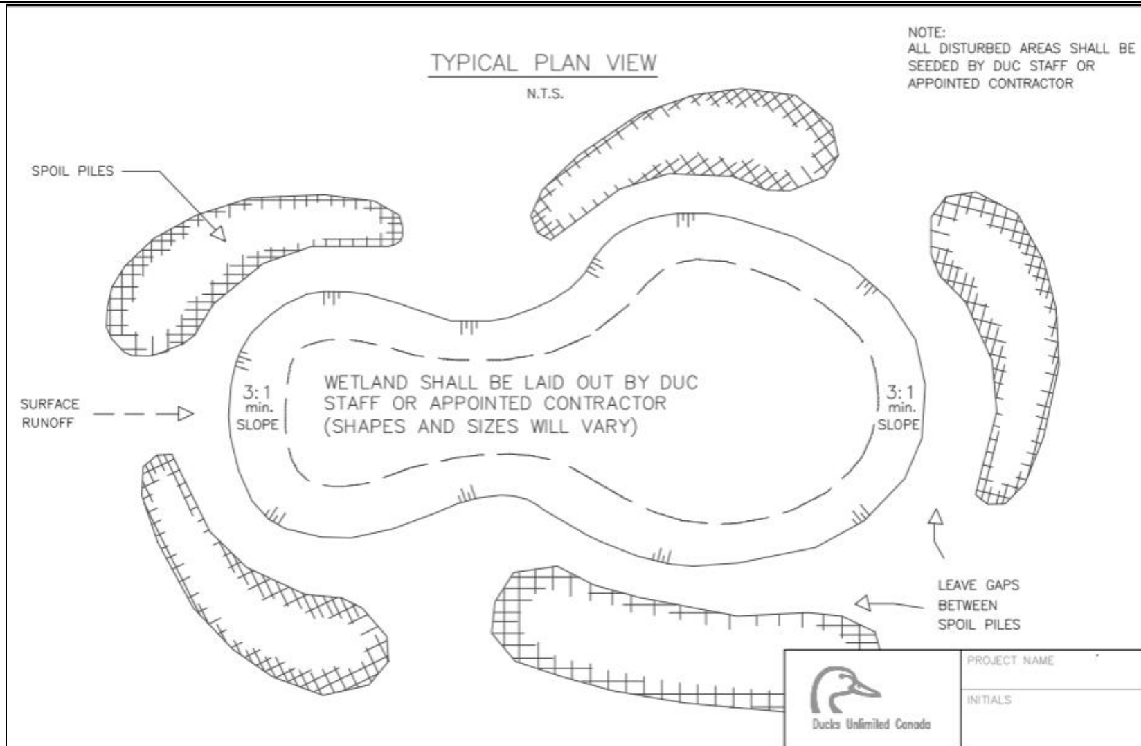
Figure 2: Overhead view of a typical excavated wetland
